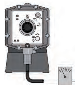
Control type: “Analogue” Stroke length adjustment 1:10, Stoke frequency control 0-100 % proportional to analogue signal 0/4-20 mA. *)
