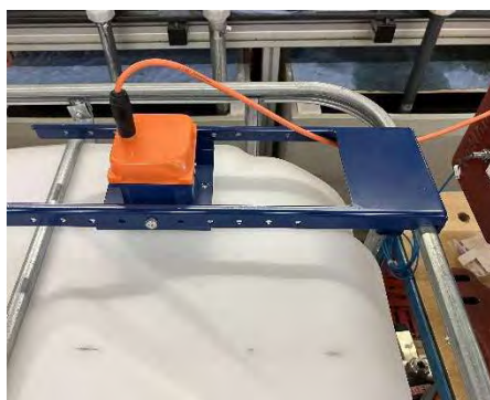
Mounting Bracket - Part No. 1130661
