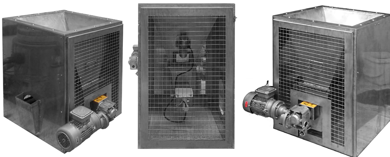
The hopper has an inspection port, and a mounting pad for a vibrator
