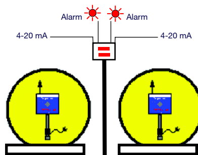
PA24022518 Twin Drum Scale & Control Unit (Digital) with alarm & 4-20 mA
