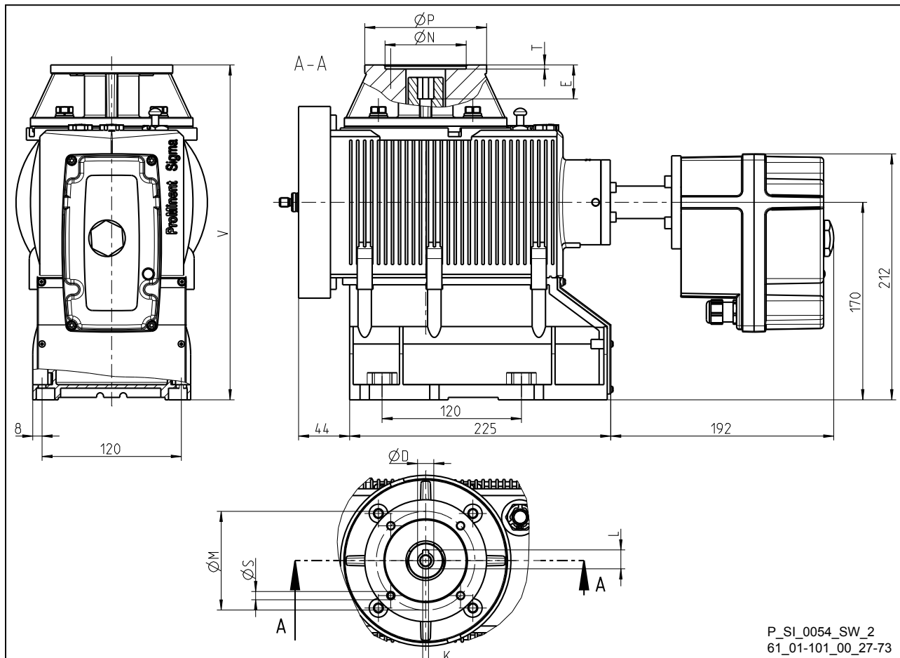
Fig. 28: Dimensions in mm - diagram is not binding.
