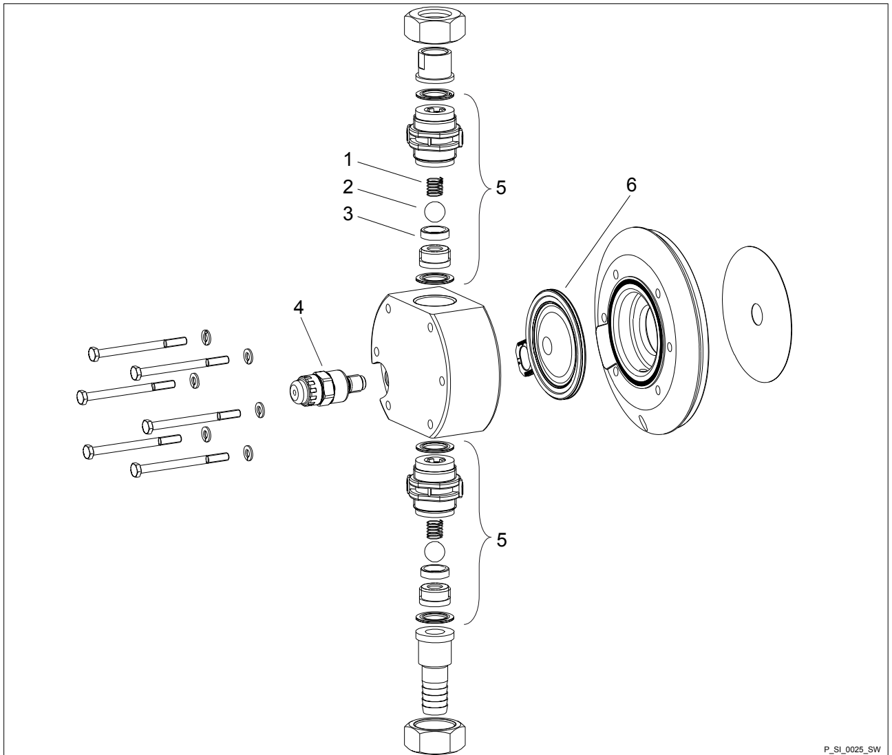
Fig. 33: Liquid end for Sigma/ 2 130 and 350 SST
