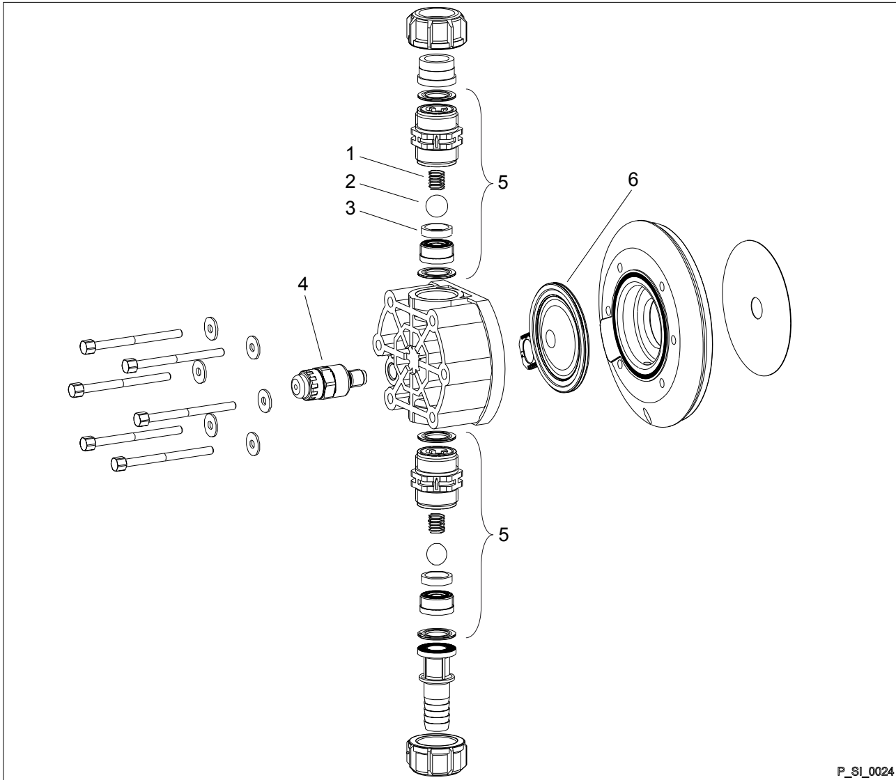
Fig. 30: Liquid end Sigma/ 2 130-DN 15 and 350-DN 25 PVT
