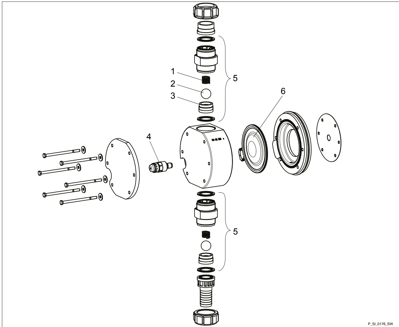
Fig. 32: Liquid end for Sigma/ 2 130 and 350 TTT
