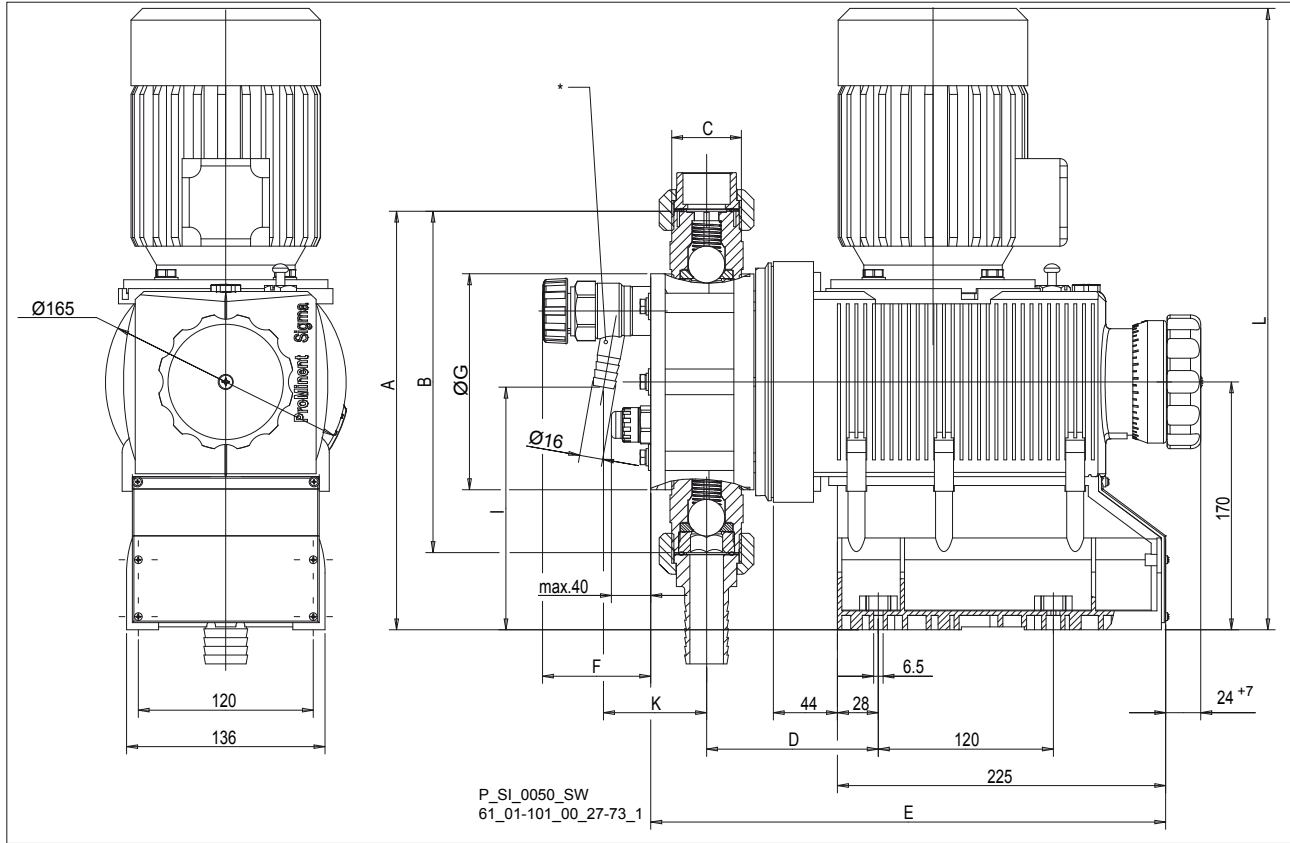
Fig. 27: Dimensions in mm - diagram is not binding.
