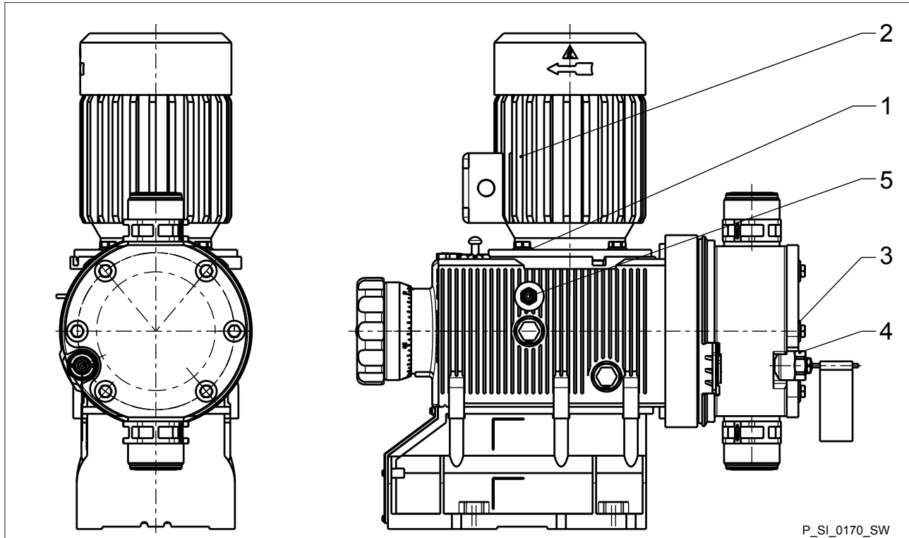
Fig. 29: Potential equalisation drawing for Sigma S2Ba
