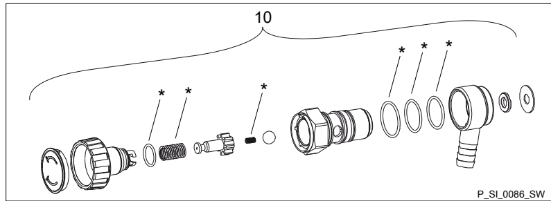
Fig. 31: Sigma/ 2 PVA relief valve-A
