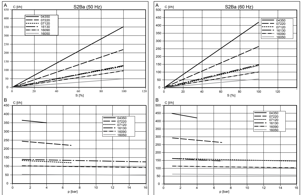
Fig. 26: A) Capacity C at minimum back pressure dependent on the stroke length s . B) Capacity C dependent on the back pressure p .
