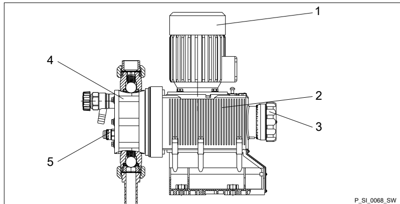
Fig. 3: Overview of equipment and control elements S2Ba
