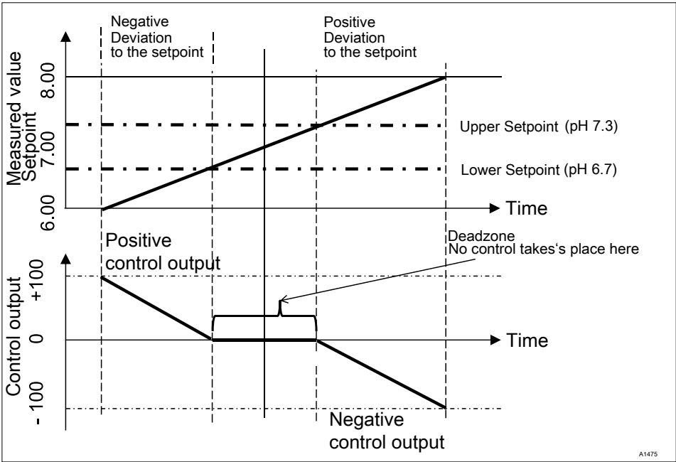
Fig. 87: Control type PID bidirectional, with neutral zone
