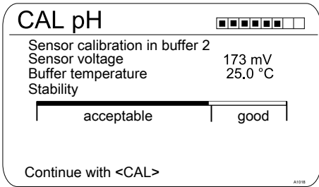
Fig. 44: Display of the sensor stability achieved
